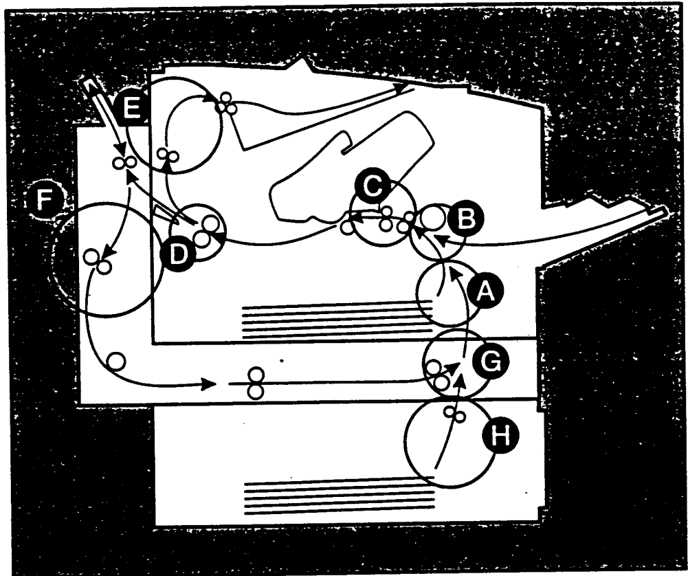
Paper Path Jam Locations
