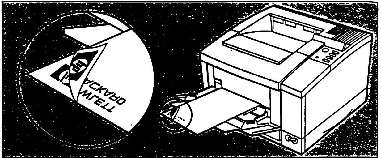
Figure 4-11 Tray 1 orientation for 2-sided printing: print-side down, bottom edge forward.
